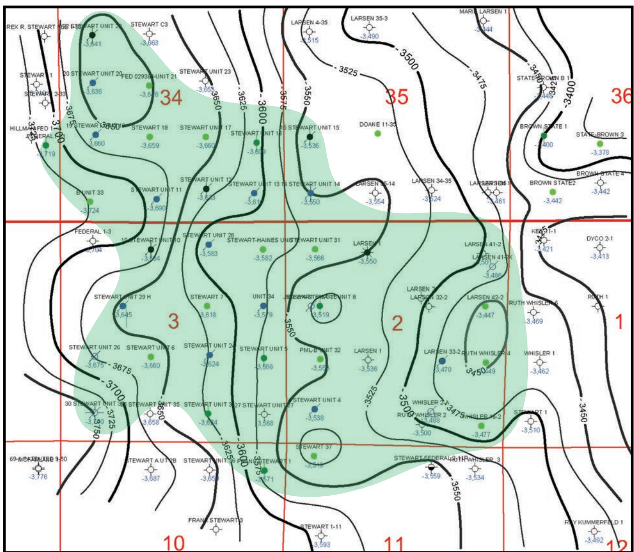
Figure 20. Base map of Stewart Field (T50 & 51N- R69W), Campbell County, Wyoming. Contours are subsea values on the top of the Minnelusa.
