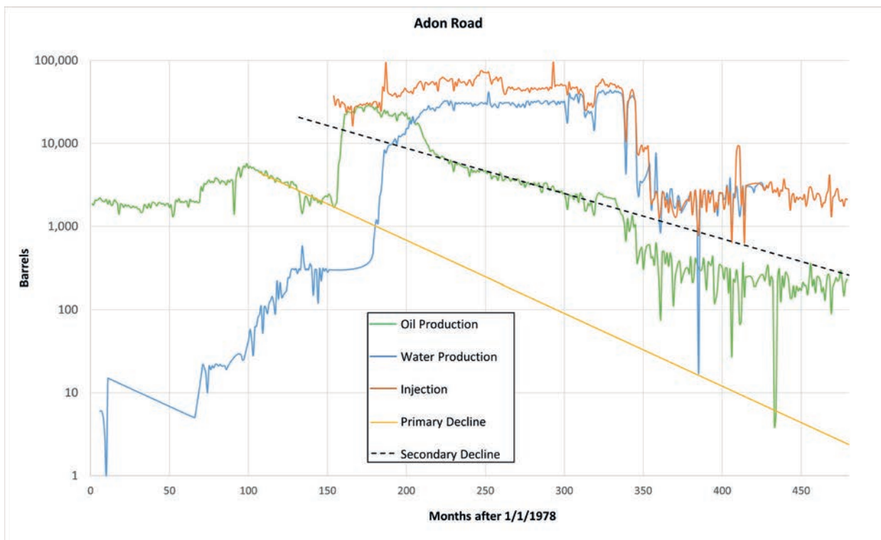
Adon Road: Polymer injection months 162 - 216.
