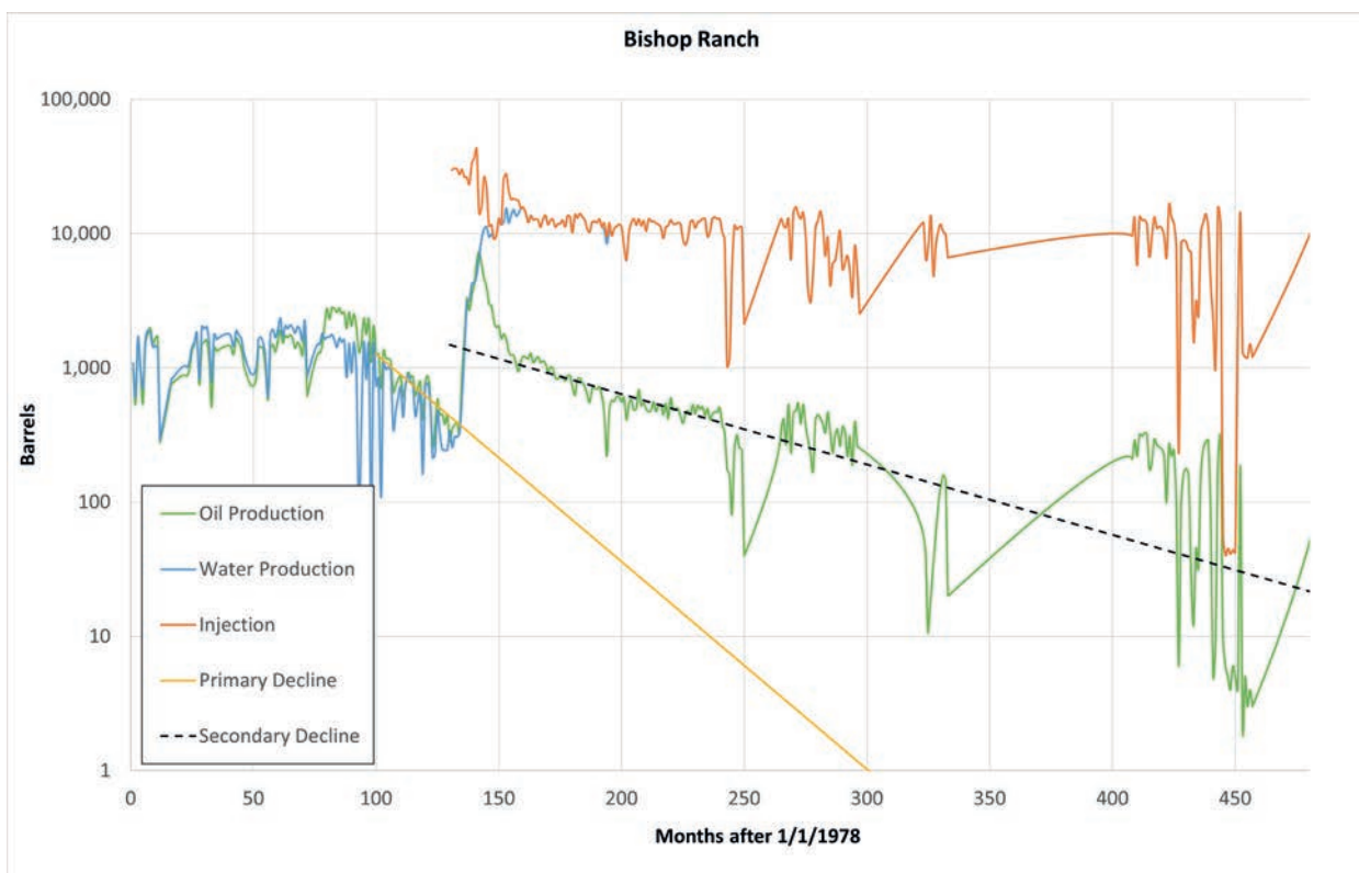
Bishop Ranch: Polymer injection months 132 - 156.
