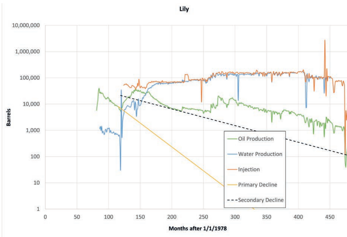
Lily: Polymer injection months 123 - 161.
