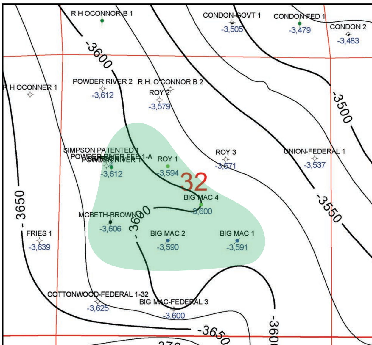
Figure 7. Big Mac Field (T52N-R69W), Campbell County, Wyoming. Contours are subsea values on the top of the Minnelusa.
