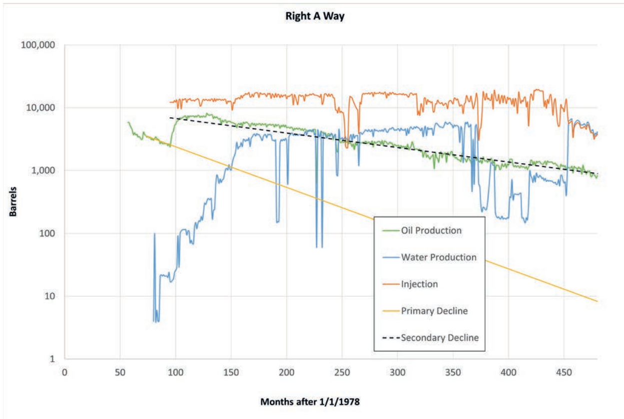
Right A Way: Polymer injection months 95 - 244.
