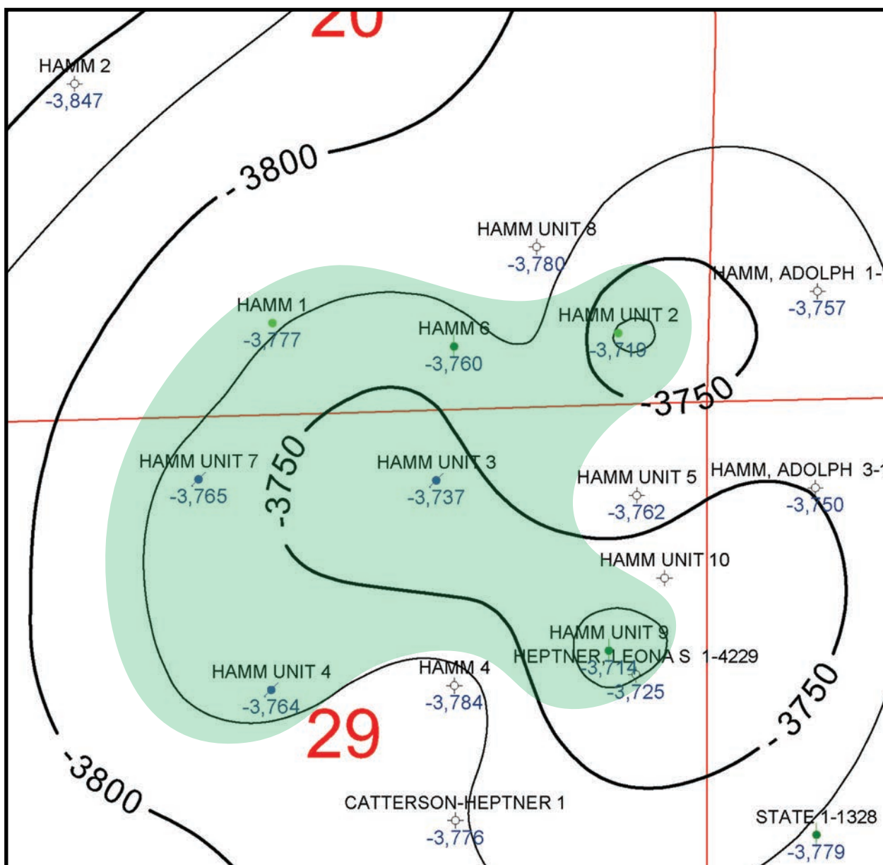
Figure 11. Hamm Field (T51N-R69W), Campbell County, Wyoming. Contours are subsea values on the top of the Minnelusa.
