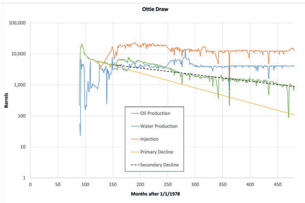
Ottie Draw: Polymer injection months 150 - 250.
